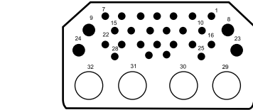
32W4M 24 #20HD, 4 #16, 4 Coaxial* Test Voltage: 1500 (Coax 1000)
