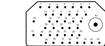
40W1M 39 #20HD, 1 Coaxial† Test Voltage: 1500 (Coax 1000)
