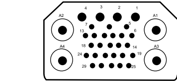
33C4M 25 #20HD, 4 Coaxial†, 4 #16 Test Voltage: 1000
