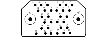
32W2M 30 #20HD, 2 Coaxial† Test Voltage: 1500 (Coax 1000)
