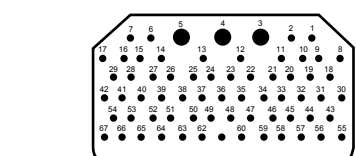
67M 64 #20HD, 3 #16 Test Voltage: 1000
