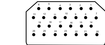
26M 26 #16 Test Voltage: 1500
