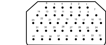
40M 40 #20HD Test Voltage: 1500
