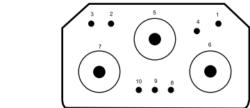
10W3M 7 #20HD, 3 Coaxial** Test Voltage: 1500 (Coax 1000)
