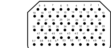
57M 57 #20HD Test Voltage: 1500
