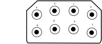
W8M 8 Coaxial* Test Voltage: 1000
