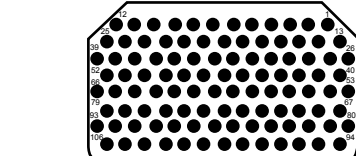
A106 106 #22 Test Voltage: 1000
