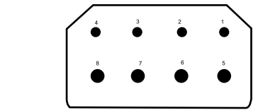
D8M 4 #16, 4 #12 Test Voltage: 1500
