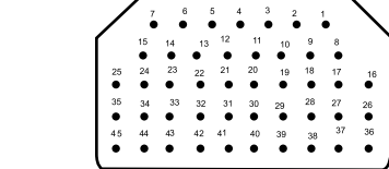
45M 45 #20HD Test Voltage: 1500
