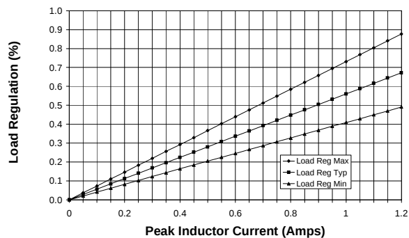
SC192 Load Regulation Limits
