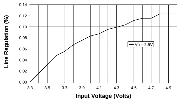
Line Regulation at I_{OUT} = 300\text{mA}
