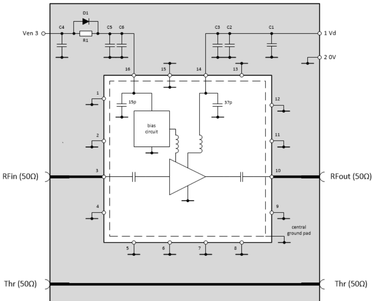
Figure 31: EV90G301 Schematic
