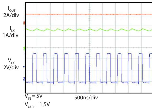
Steady State (PWM) Operation ( I_{OUT} = 2A )
