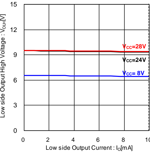
Figure 15. Low side Output High Voltage vs Low side Output Current (Ta=25°C)
