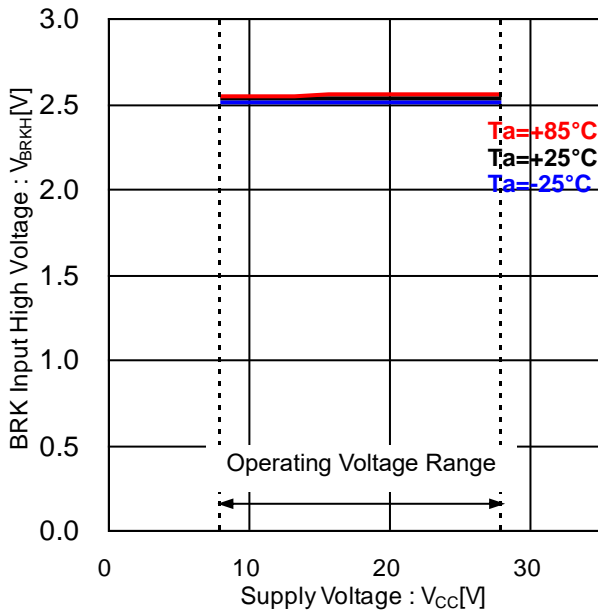
Figure 29. BRK Input High Voltage vs Supply Voltage
