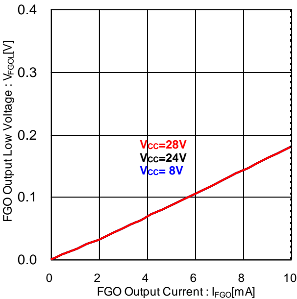
Figure 37. FGO Output Low Voltage vs FGO Output Current (Ta=25°C)
