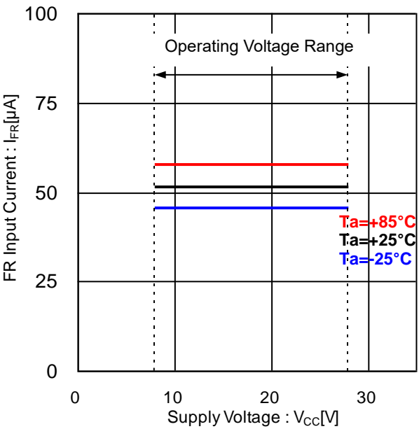
Figure 25. FR Input Current vs Supply Voltage
