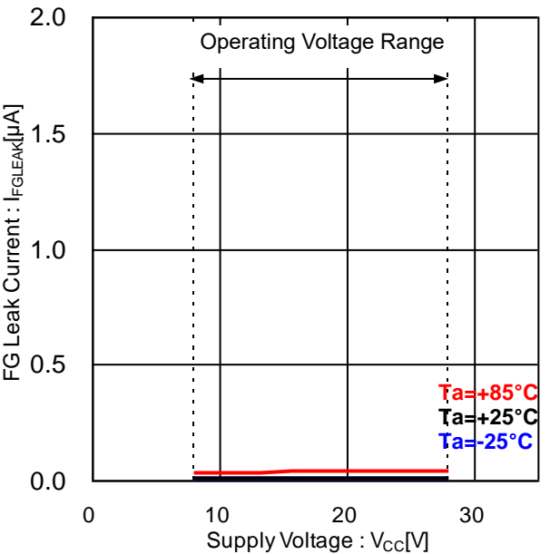
Figure 38. FG Leak Current vs Supply Voltage
