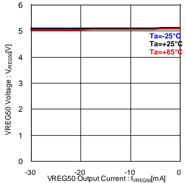
Figure 7. VREG50 Voltage vs VREG50 Output Current ( V_{CC}=24V )
