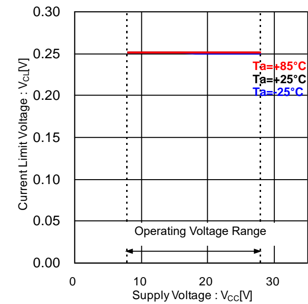
Figure 40. Current Limit Voltage vs Supply Voltage
