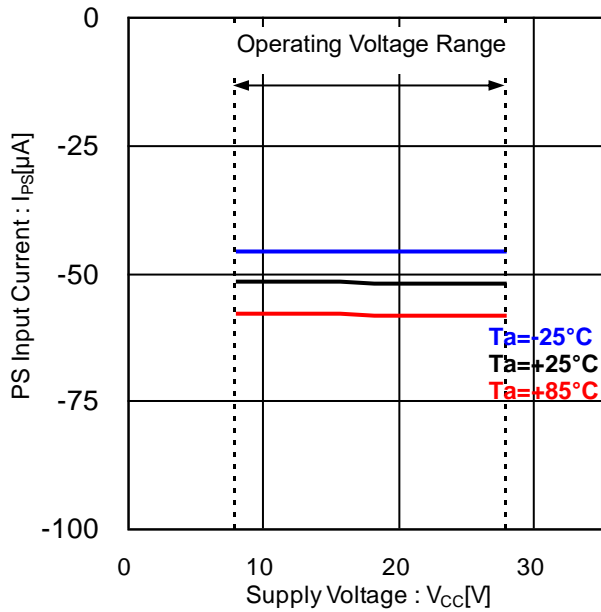
Figure 22. PS Input Current vs Supply Voltage
