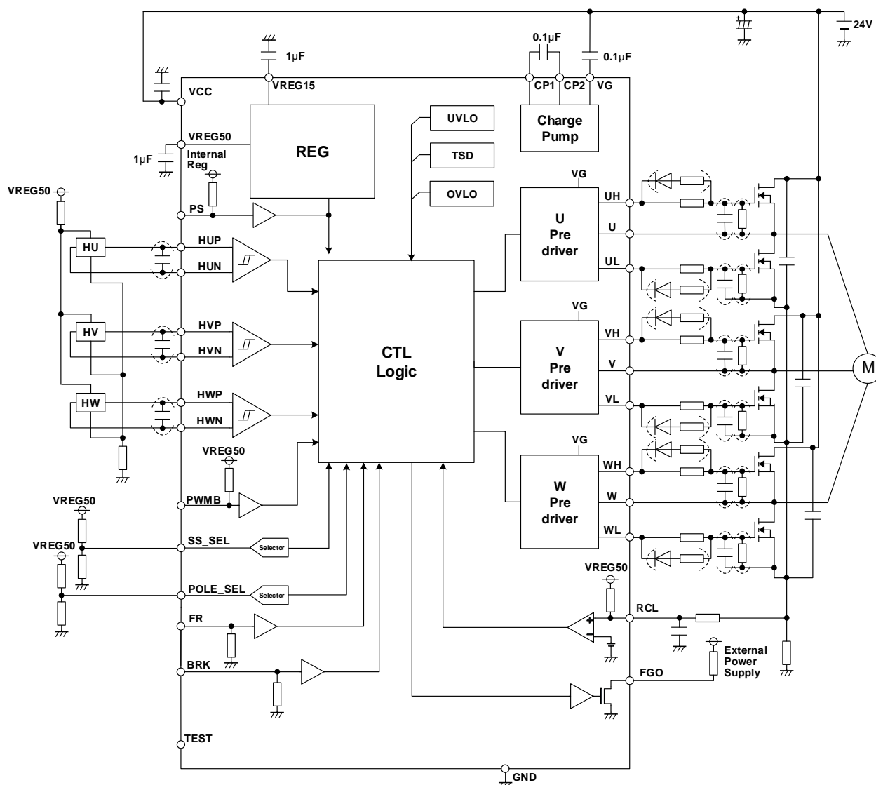
Figure 3. Application example
