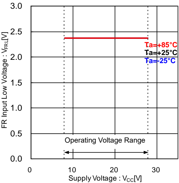
Figure 27. FR Input Low Voltage vs Supply Voltage
