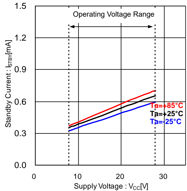
Figure 5. Standby Current vs Supply Voltage
