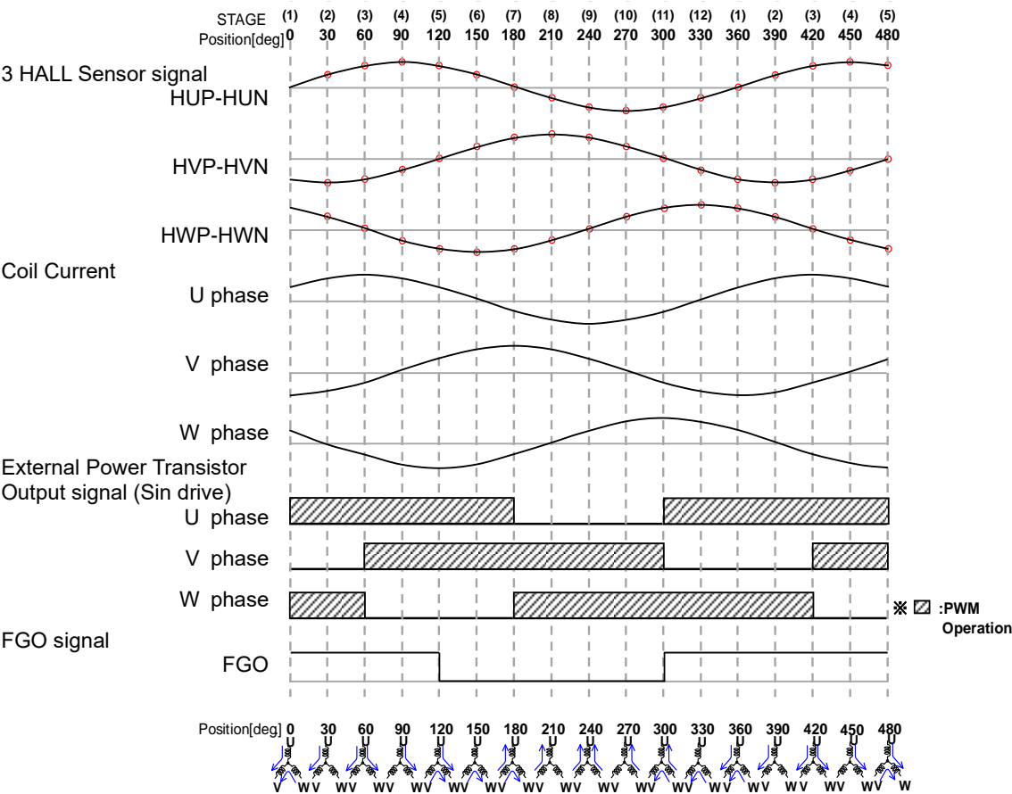
Figure 41. Timing Chart of Hall Detection Drive (FR=High)
