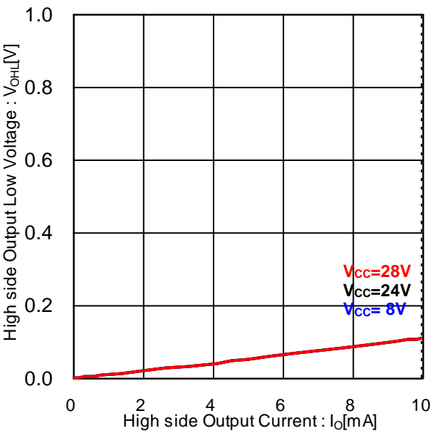
Figure 13. High side Output Low Voltage vs High side Output Current (Ta=25°C)
