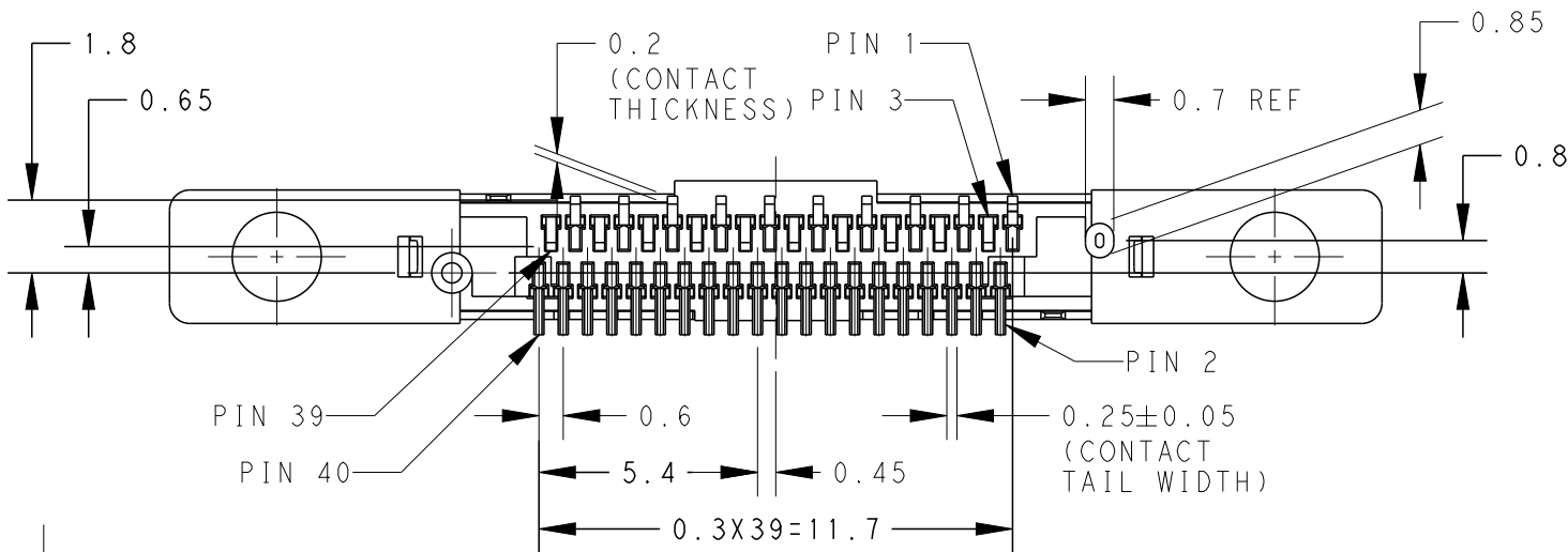
VIEW C
