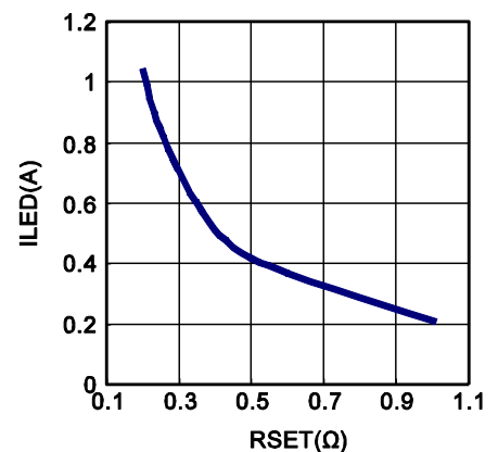
I_{LED} vs. R_{set}
