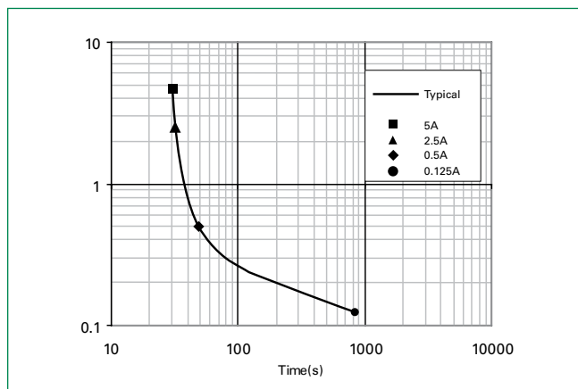
Figure 1. Thermal Characteristics
