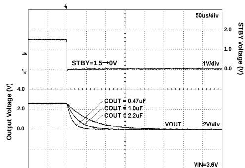
Fig 153. Discharge Time
