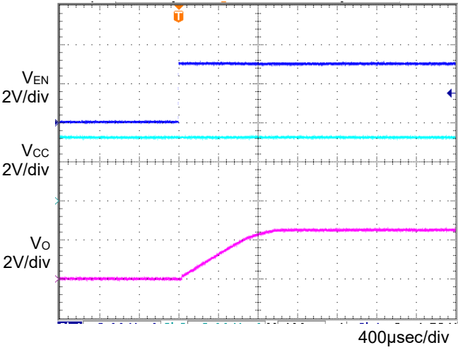
Fig.16 Input sequence 2 Co=1µF,Ta=25°C
