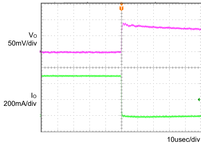
Fig.6 Transient Response (0.5 \rightarrow 0A) Co=1 \mu F, Ta=-40°C
