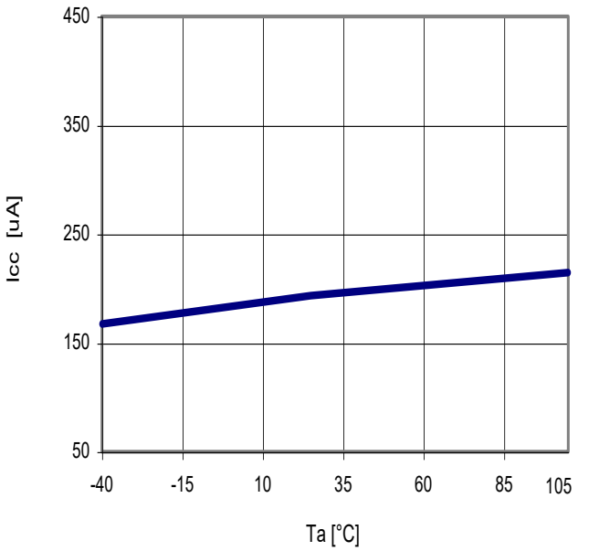
Fig.22 T_a - I_{cc}
