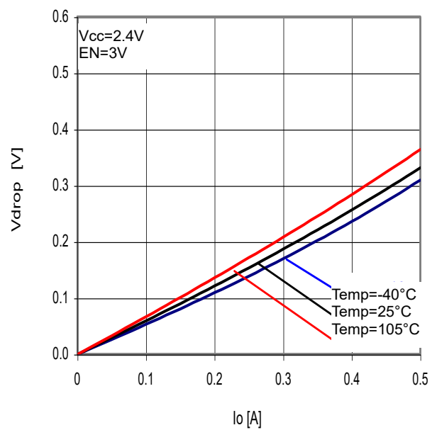
Fig.34 Minimum dropout Voltage 1 ( V_{CC}=2.4\text{V} )
