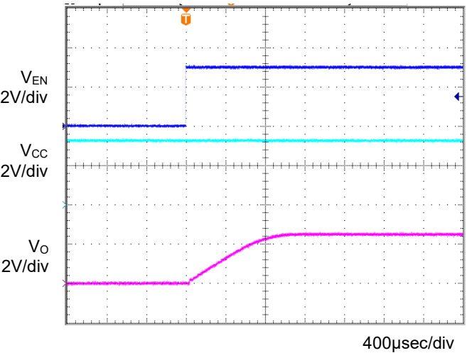
Fig.17 Input sequence 2 Co=1µF,Ta=105°C
