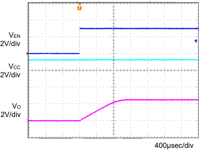
Fig.15 Input sequence 2 Co=1µF,Ta=-40°C
