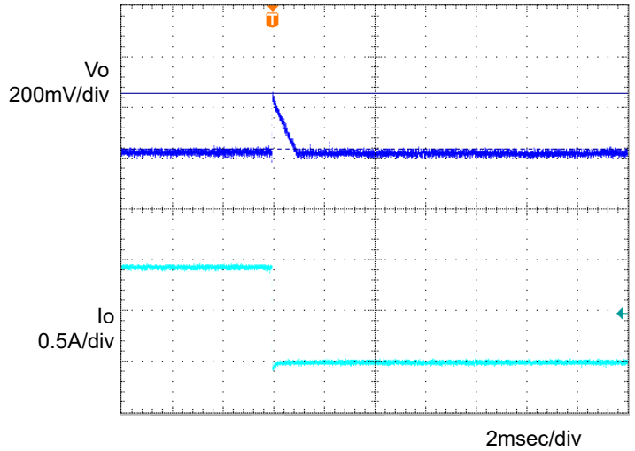
Fig.6 Transient Response (1.0→0A) Co=1\mu F, Ta=-40^{\circ}C
