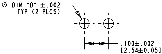
RECOMMENDED P.C.B. HOLE PATTERN
