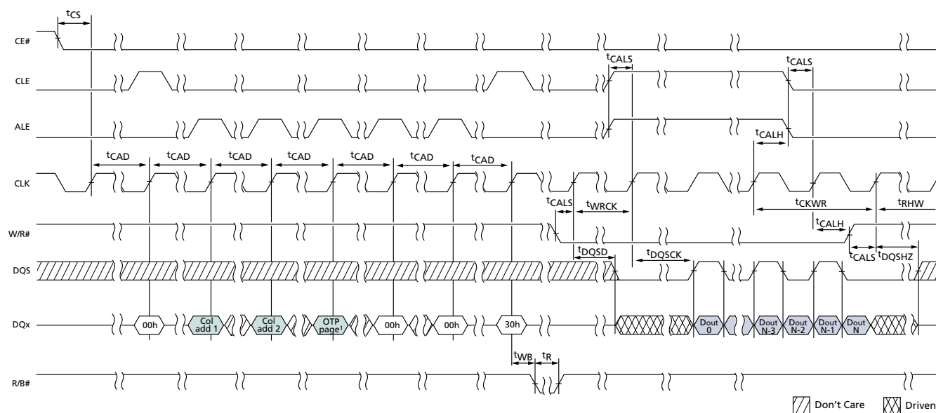
Figure 119: READ OTP PAGE
