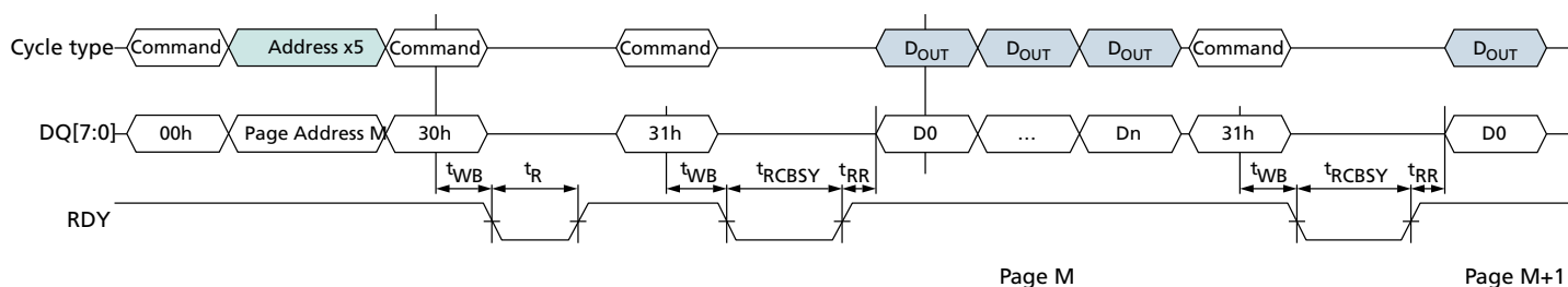
Figure 57: READ PAGE CACHE SEQUENTIAL (31h) Operation
