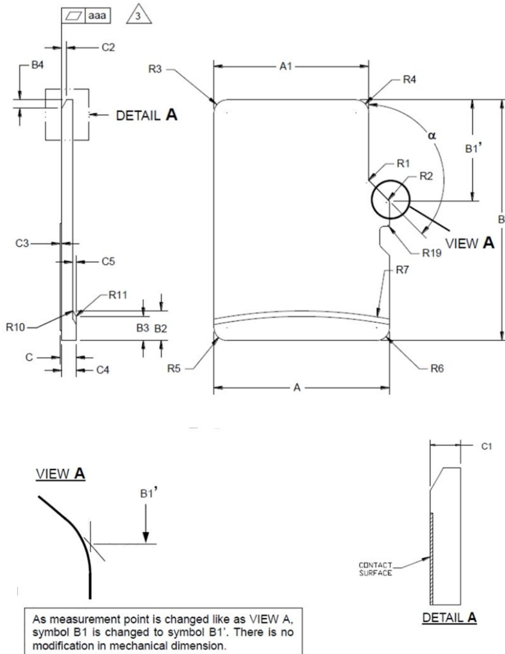
Figure 10: Top View
