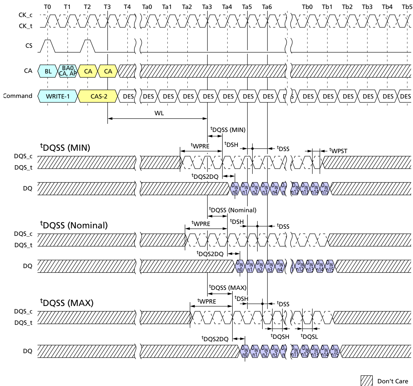
Figure 30: Write Timing
