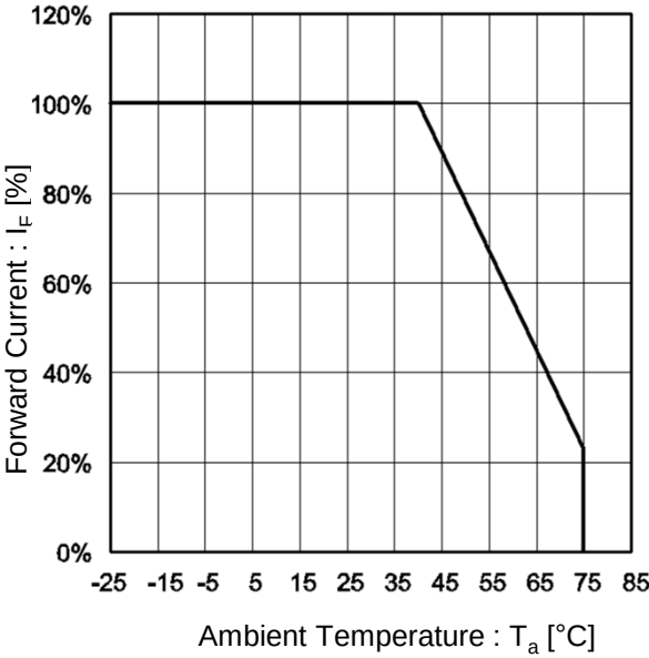
Fig.6 Derating
