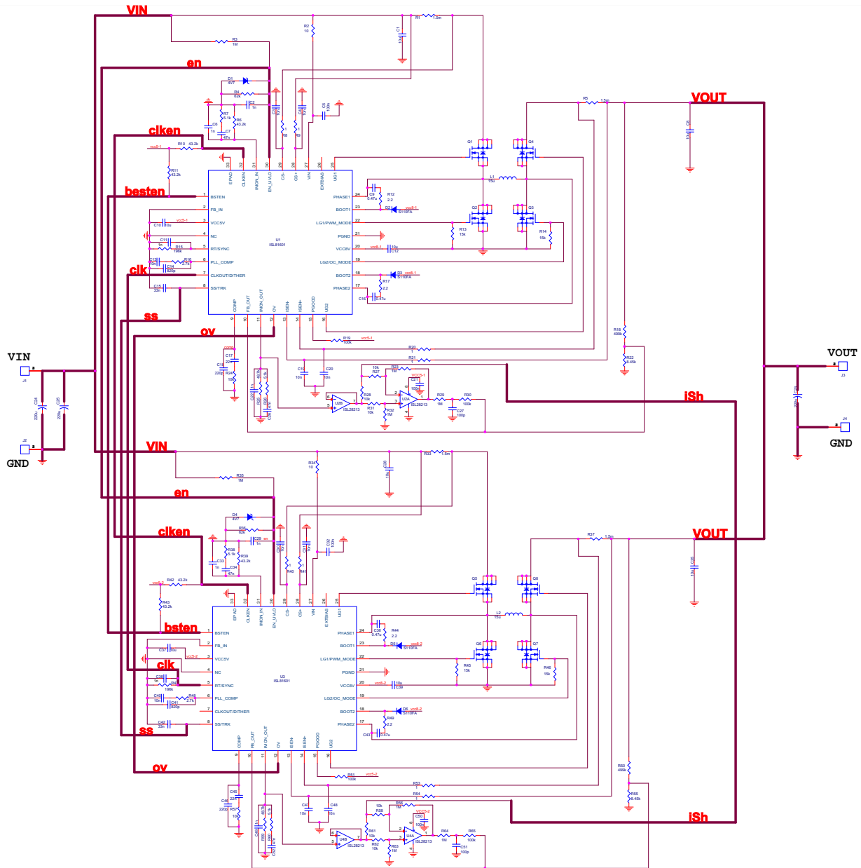
Figure 54. ISL81601DEMO12 Current Sharing Circuit
