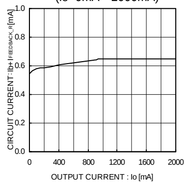
Fig.9 Circuit Current ( I_{\text{FEEDBACK\_R}} \approx 75\mu\text{A} )
