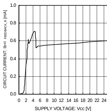
Fig.1 Circuit Current ( I_{\text{FEEDBACK\_R}} \approx 75\mu\text{A} )
