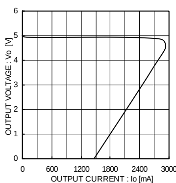
Fig.5 Load Regulation
