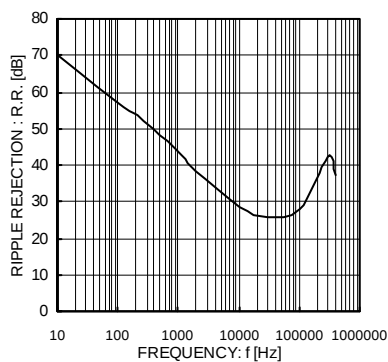
Fig.7 Ripple Rejection
