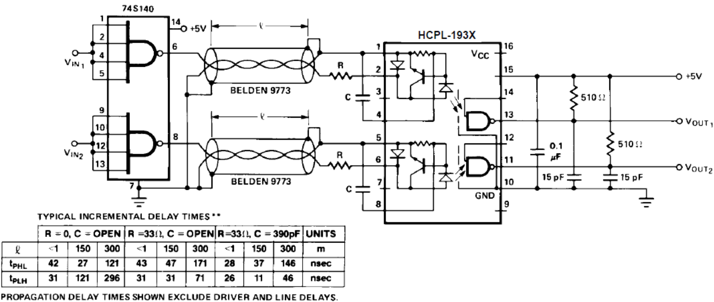
Figure 12 Polarity Reversing, Split Phase
