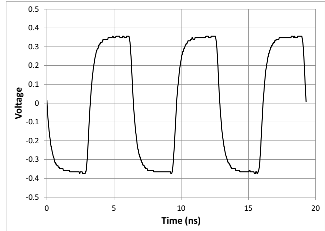
Typical Waveform at 155.52 MHz
