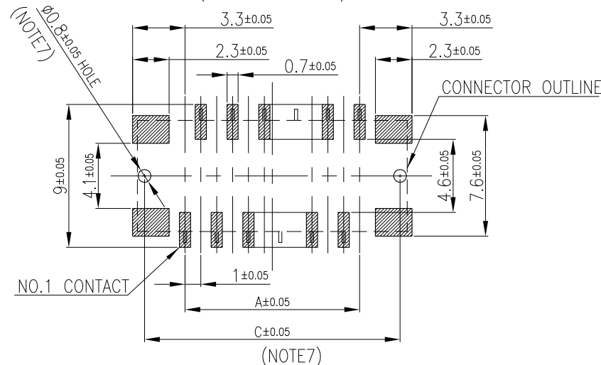
RECOMMENDED PC BOARD LAYOUT (COMPONENT SIDE)
