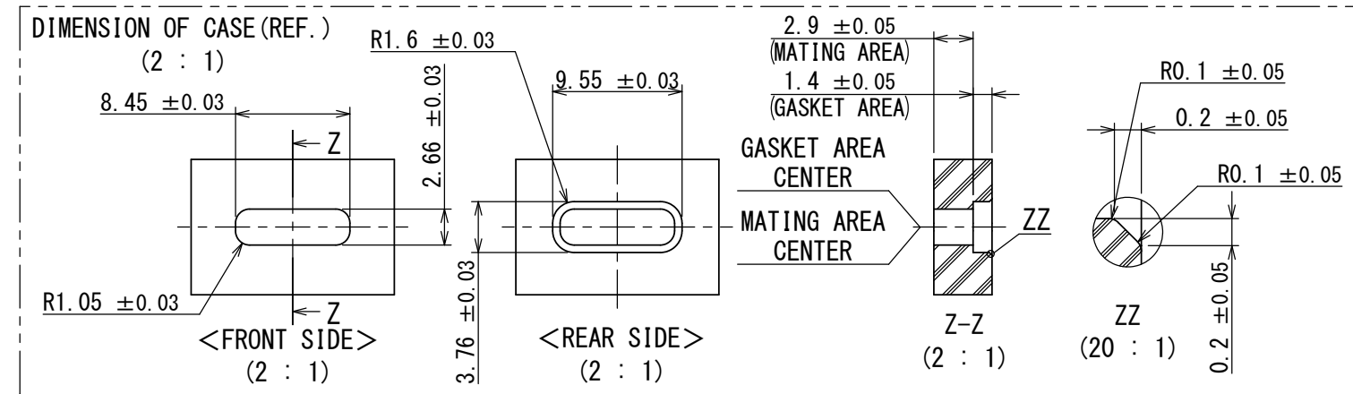
APPEARANCE (REF.) (5 : 1)
