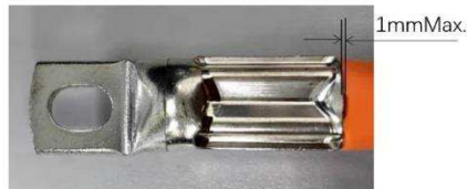
Figure 7: ring tongue crimp
