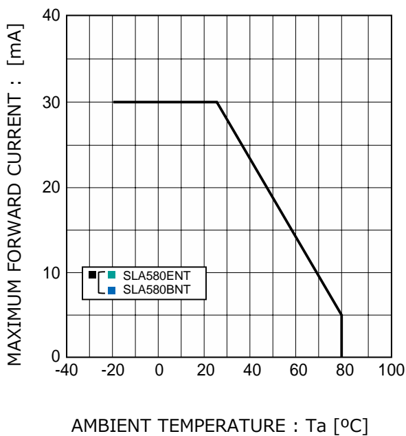
Fig.4 Derating
