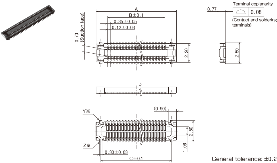
Dimension table
