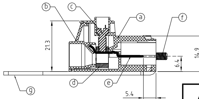
SECTION P-P
