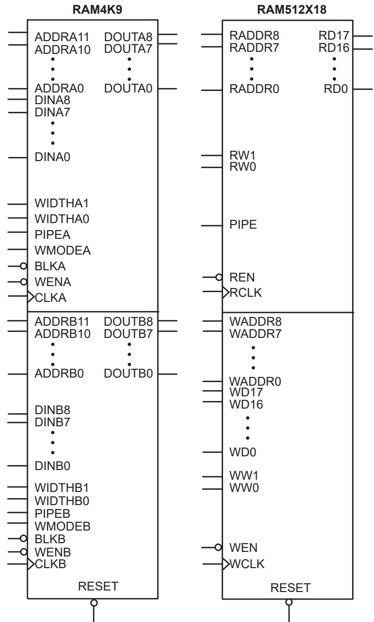
FIGURE 2-30: RAM MODELS
