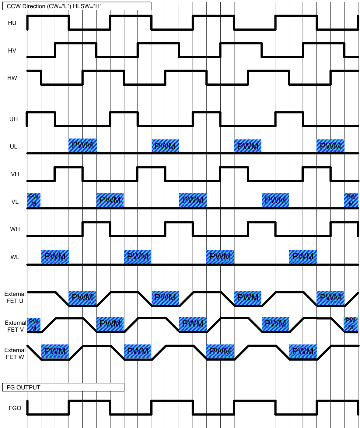
Figure 8. Timing Chart 2
