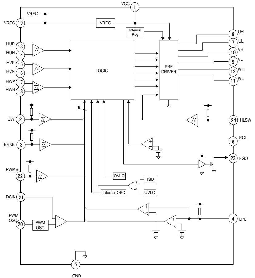
Figure 5. Block Diagram
