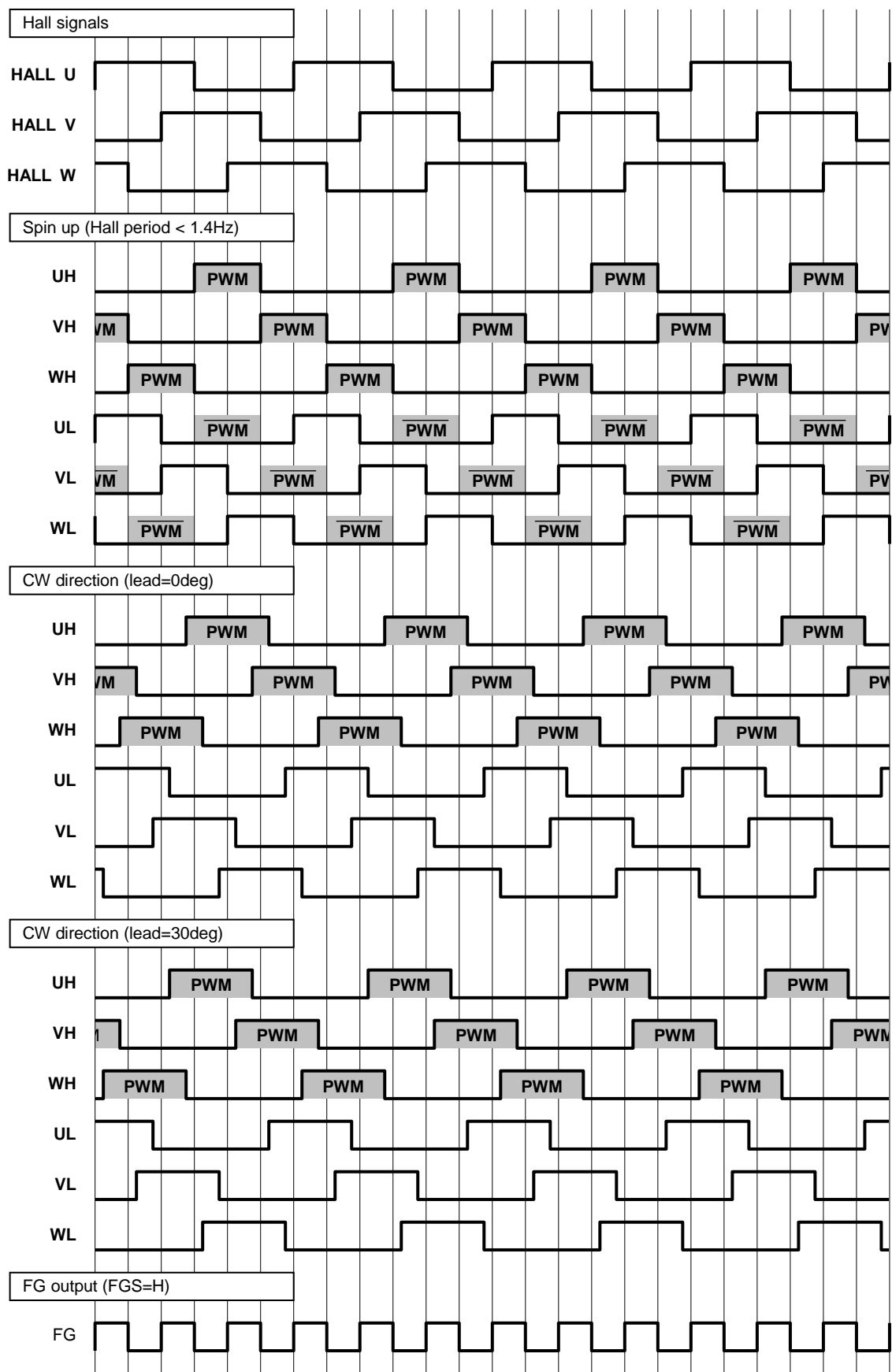
Timing Chart (CW, SQB = H)
