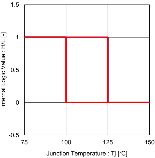
Figure 43 Thermal Shutdown
