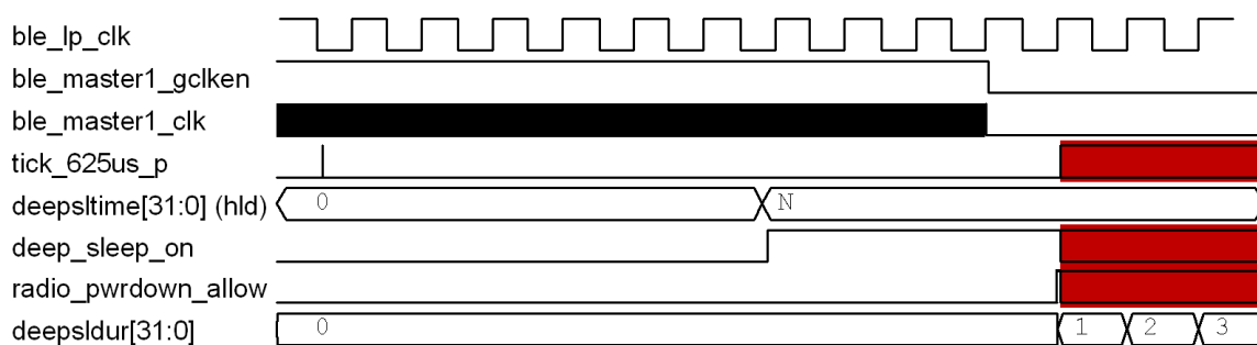
Figure 76. Entering Bluetooth® LE Deep Sleep mode
