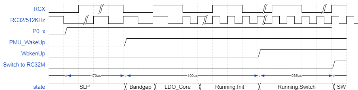
Figure 11. Wake-up (buck)
