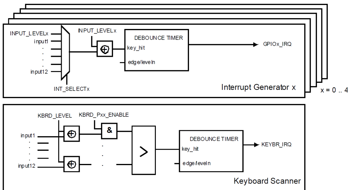
Figure 62. Keyboard controller block diagram
