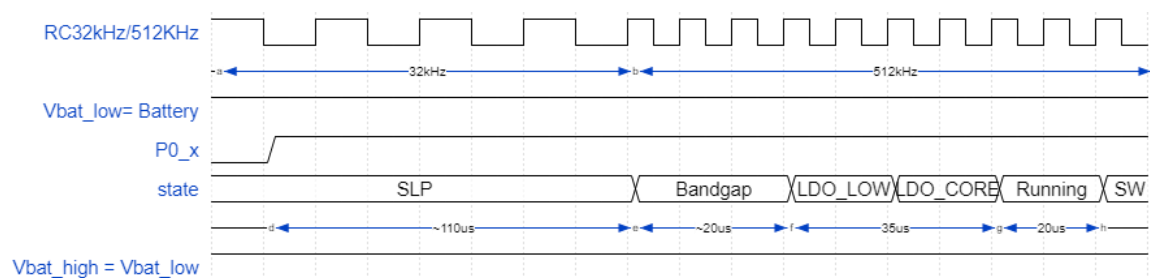
Figure 10. Wake-up from Hibernation (buck)
