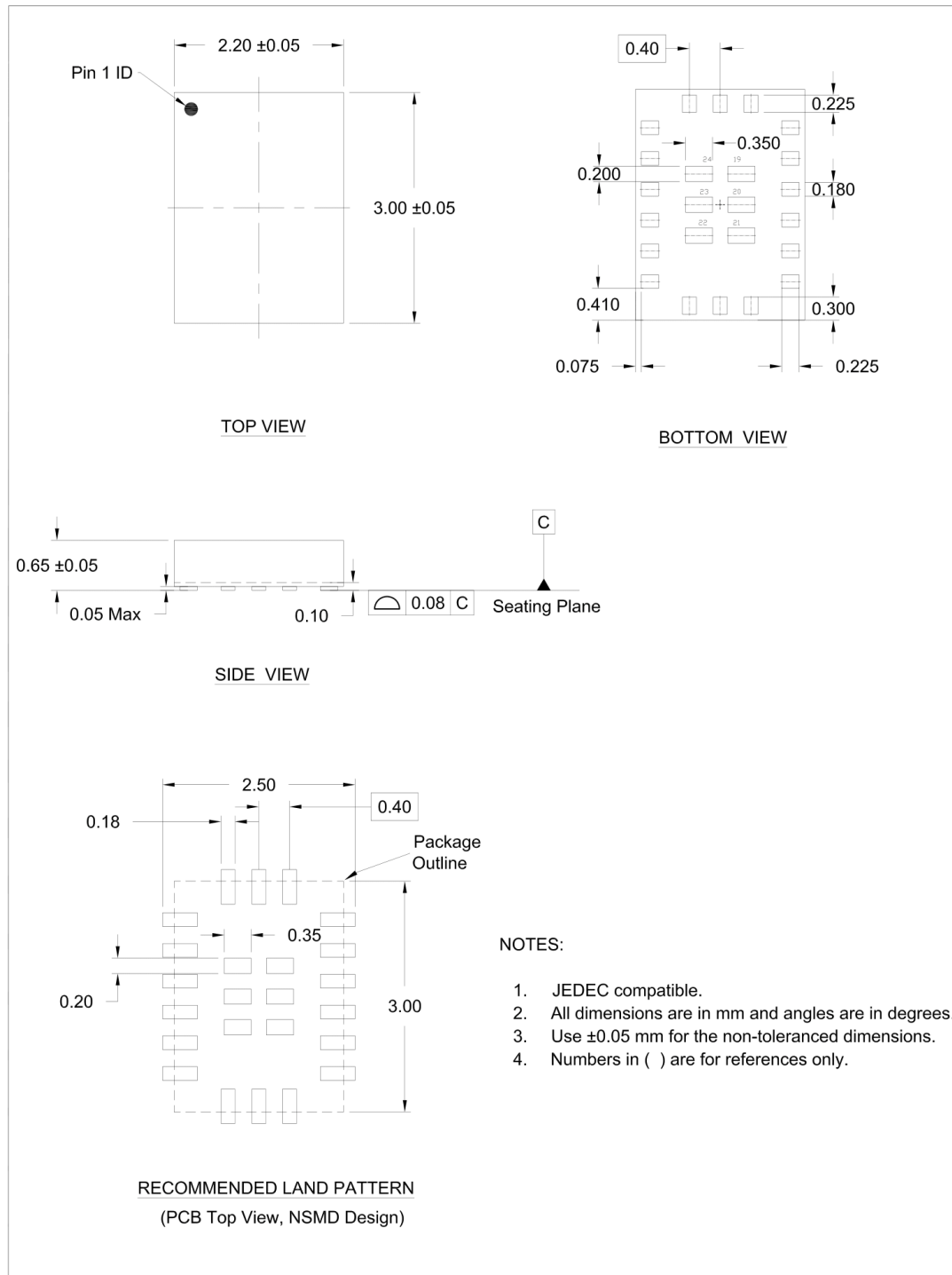
Figure 82. FCGQFN24 package outline drawing
