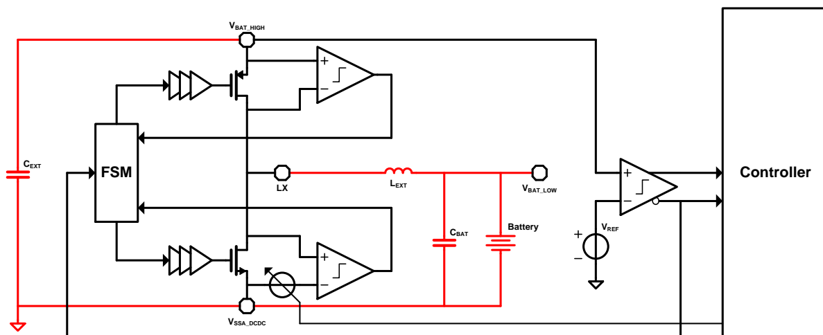
Figure 72. DCDC block diagram – boost configuration
