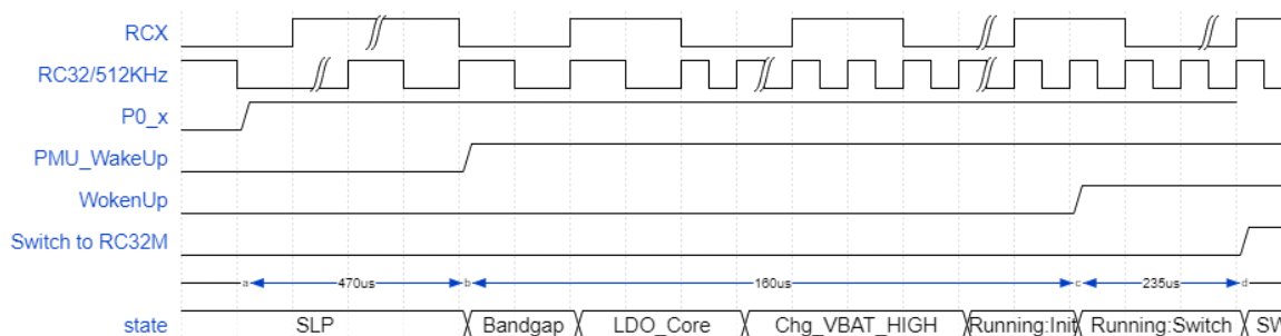
Figure 14. Wake-up from extended/deep sleep (boost)
