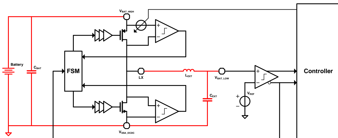
Figure 71. DCDC block diagram – buck configuration
