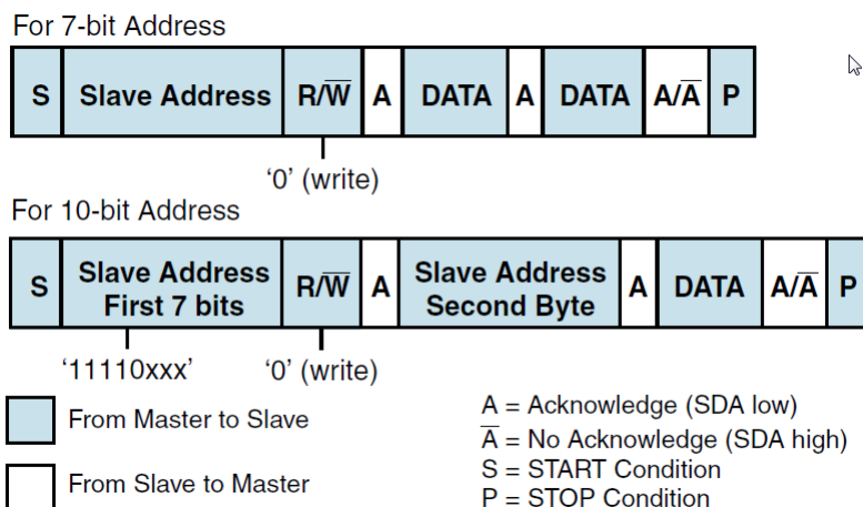
Figure 36. Master-transmitter protocol
