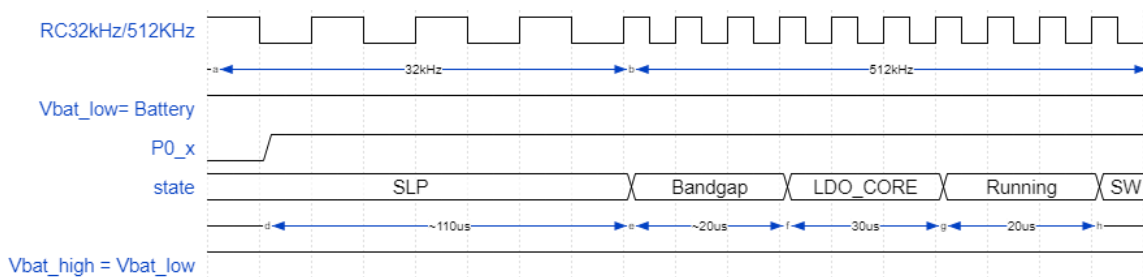
Figure 13. Wake-up from hibernation (boost)
