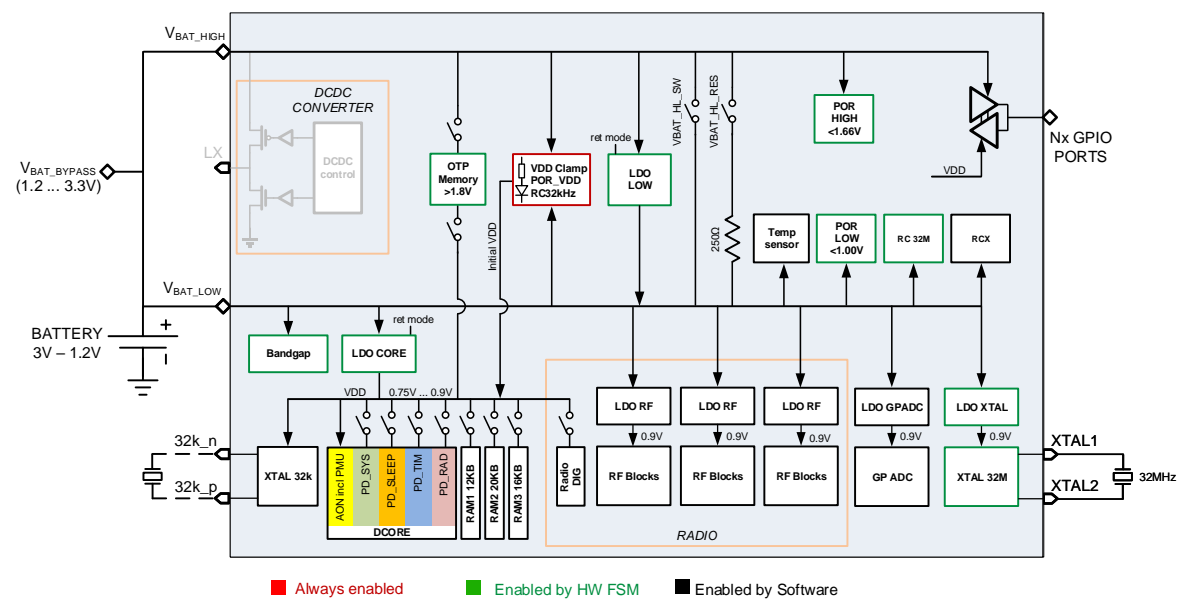
Figure 6. Power management unit: bypass configuration
