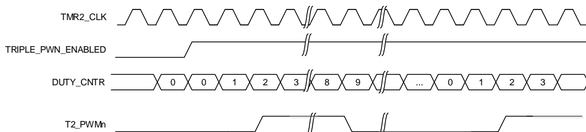
Figure 59. Timer 2 timing diagram
