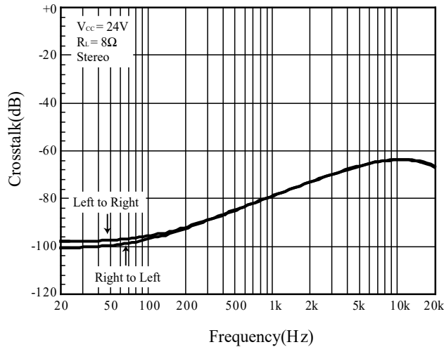
Figure 22 Cross-Talk
