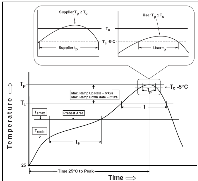
Figure 39 Classification Profile
