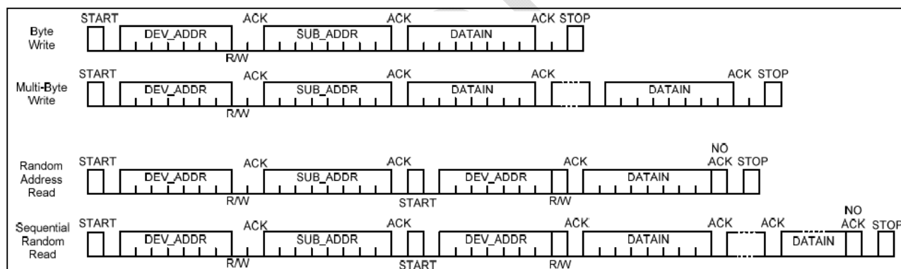
Figure 35 Data Transferring
