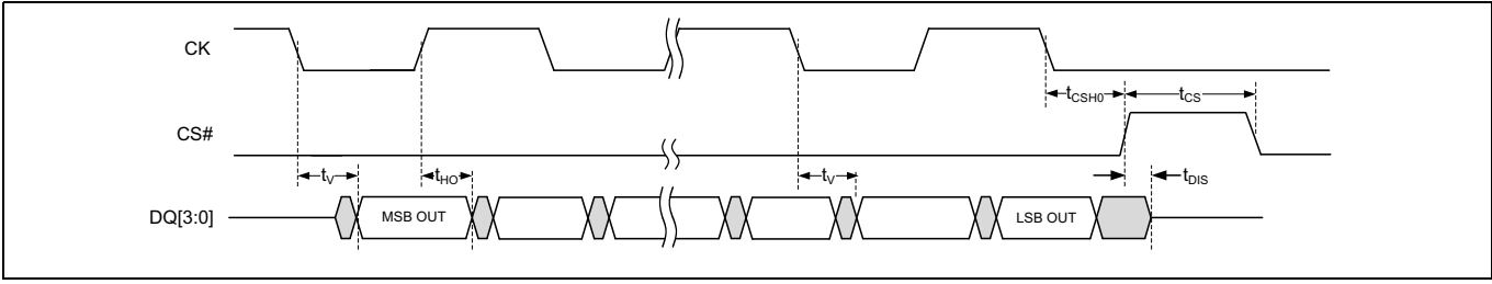
Figure 84 Quad and QPI DDR output timing
