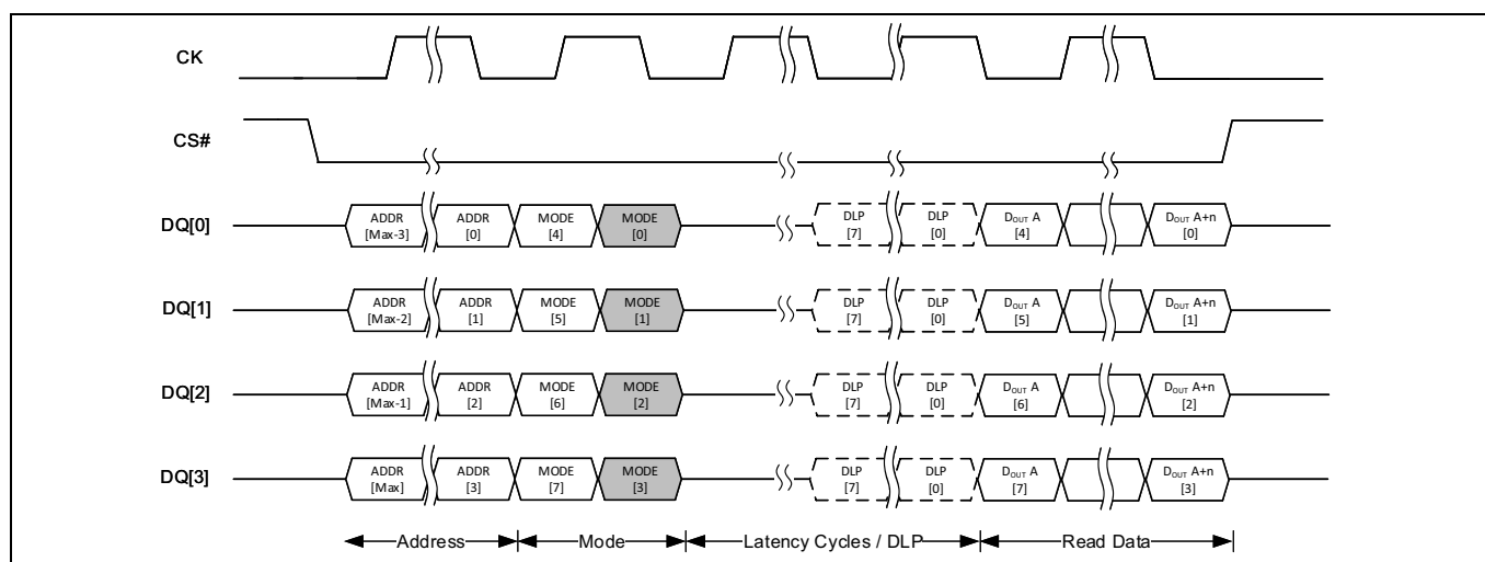
Figure 22 QIO DDR continuous read transaction with address and mode input (output latency)
