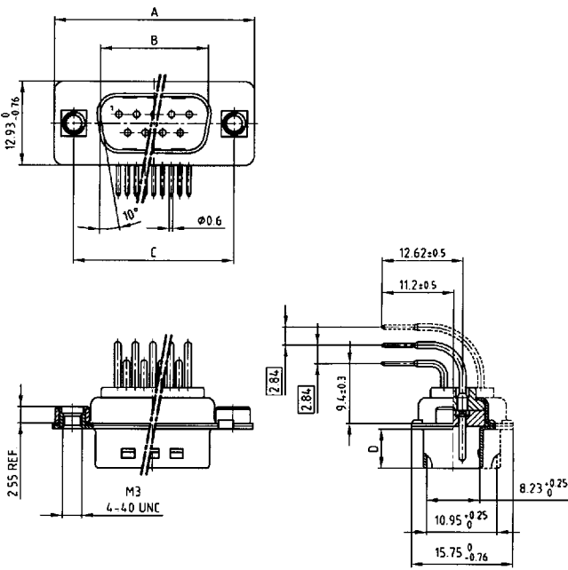
Plug connector
