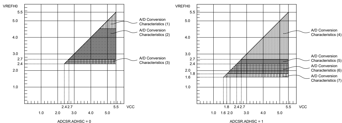
Figure 2.44 VCC0 to VREFH0 voltage range
