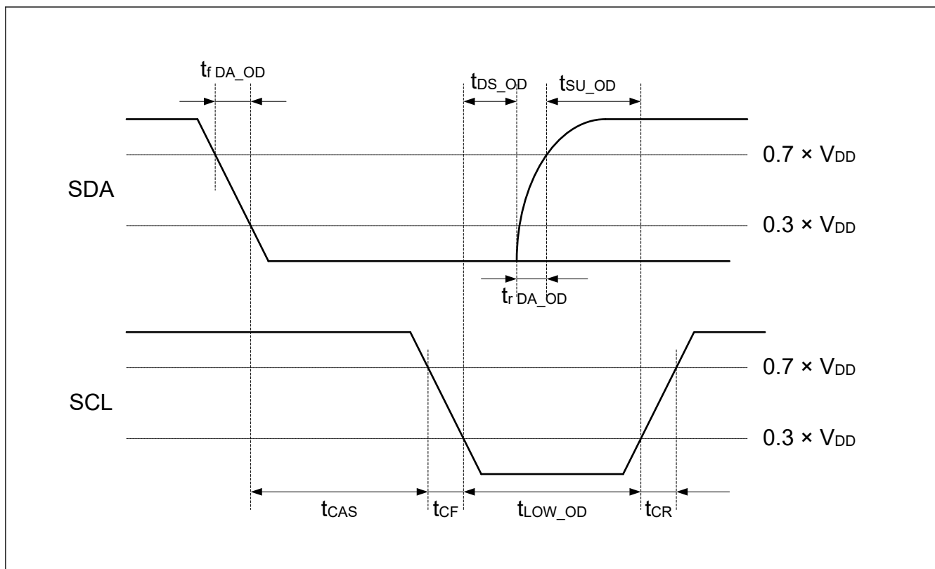
Figure 2.36 I3C START condition Timing
