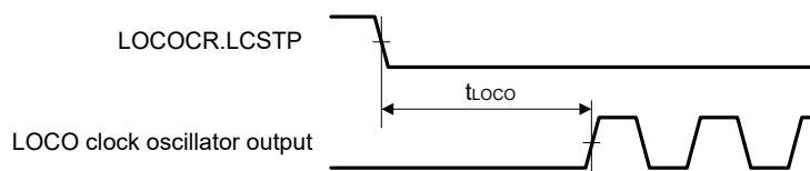
Figure 2.3 LOCO clock oscillation start timing
