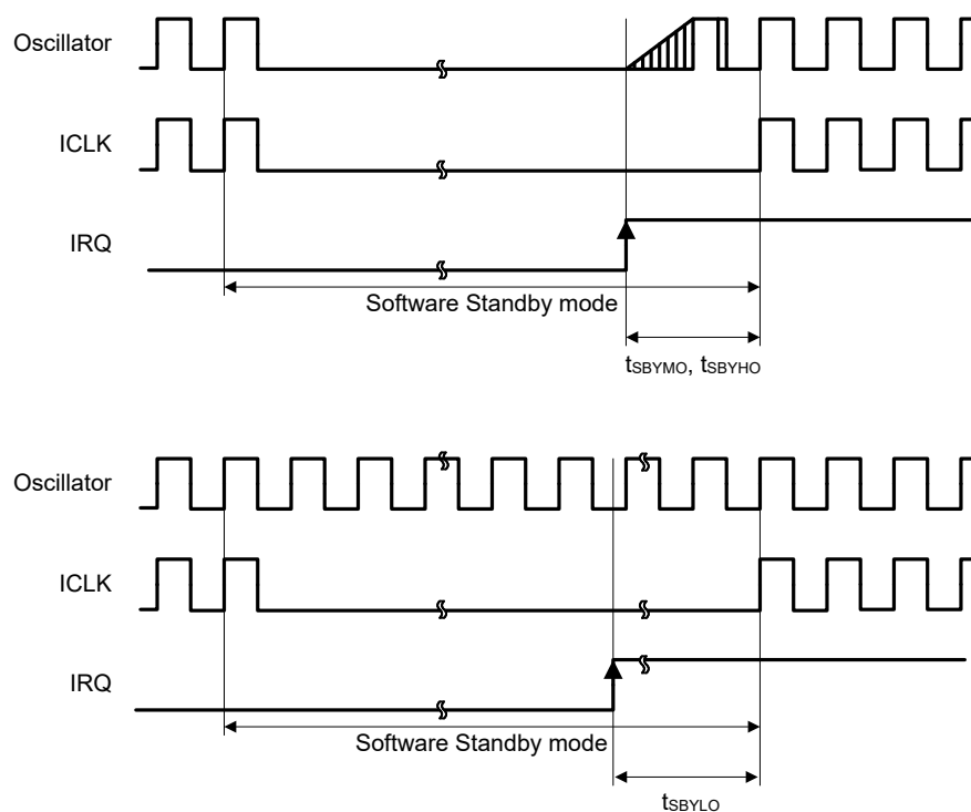
Figure 2.8 Software Standby mode cancellation timing
