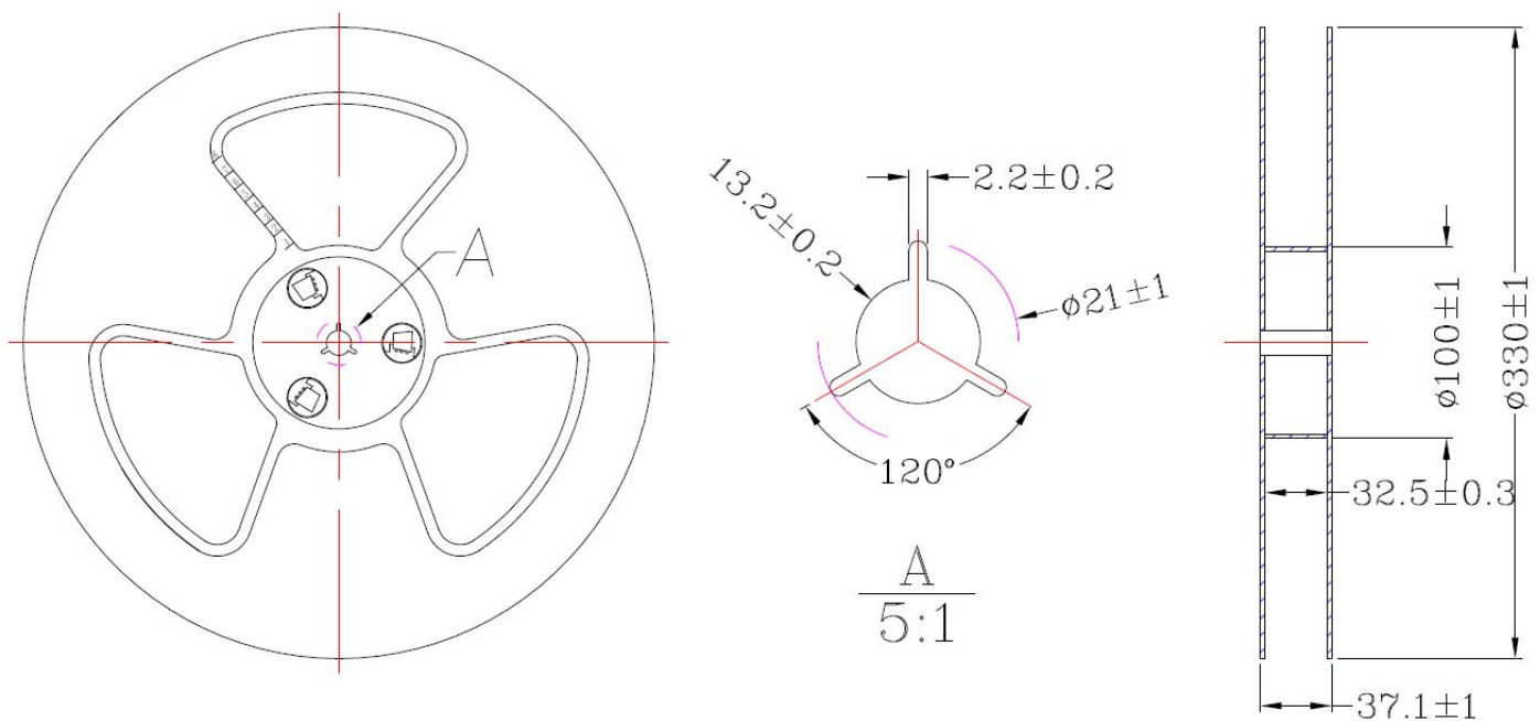
Figure 10.2. Reel Dimensions
