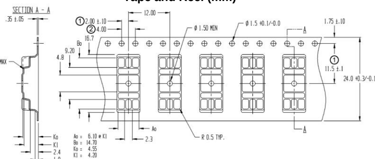
Figure 3. Packaging Dimensions (For reference only.)
