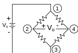
Figure 1. Excitation Schematic (Excitation 5 Vdc Typ., 6 Vdc max.)
