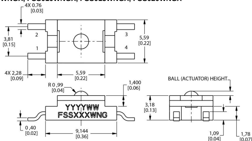
Figure 2. Sensor Mounting Diagram (For reference only: mm/[in.]
