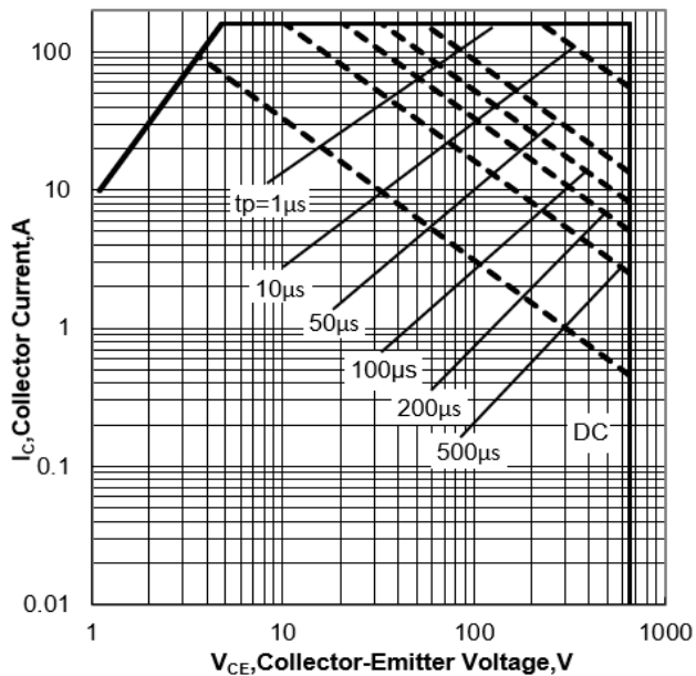
Figure 1. Forward Bias Safe Operating Area for TO247/TO220F
