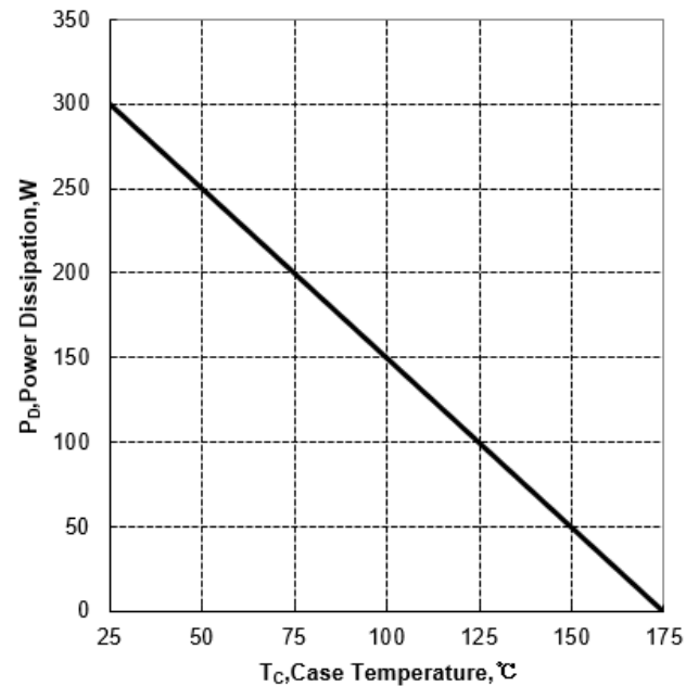
Figure 2. Power Dissipation vs Case Temperature for TO247/TO220F
