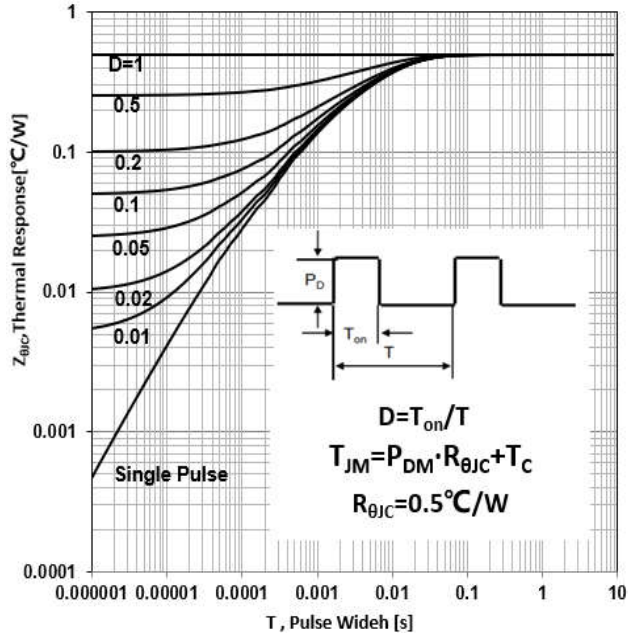
Figure 19. IGBT Transient Thermal Impedance vs Pulse Width(TO247/TO220F)
