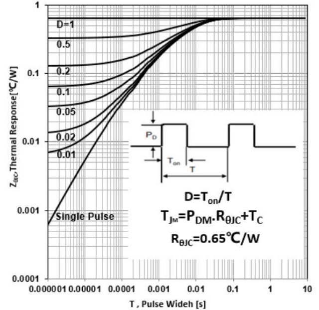
Figure 20. Diode Transient Thermal Impedance vs Pulse Width(TO247/TO220F)
