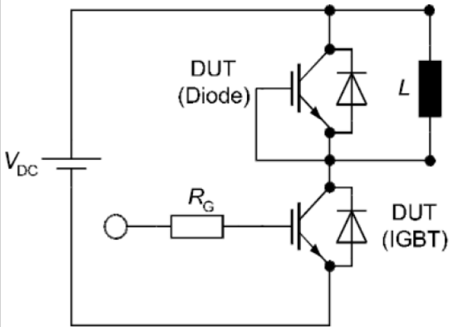
Figure 1. Inductive Switching Test Circuit
