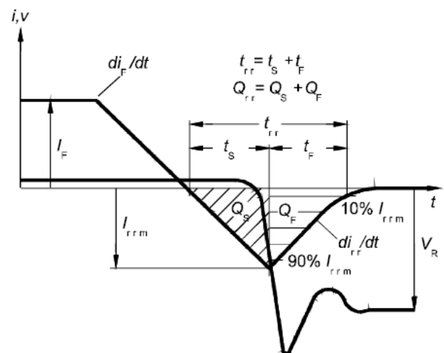
Figure 4. Definition of diode switching characteristics
