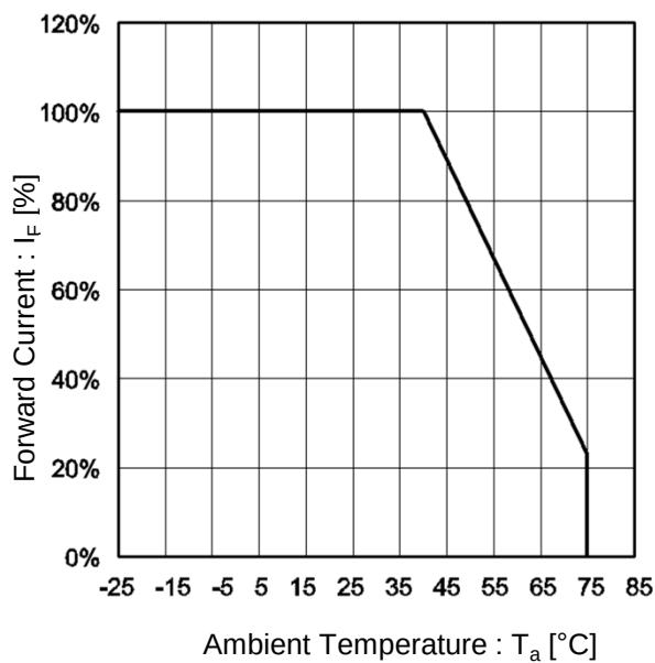
Fig.7 Derating
