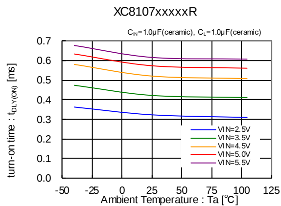
(18) turn-on time vs. Ambient Temperature
