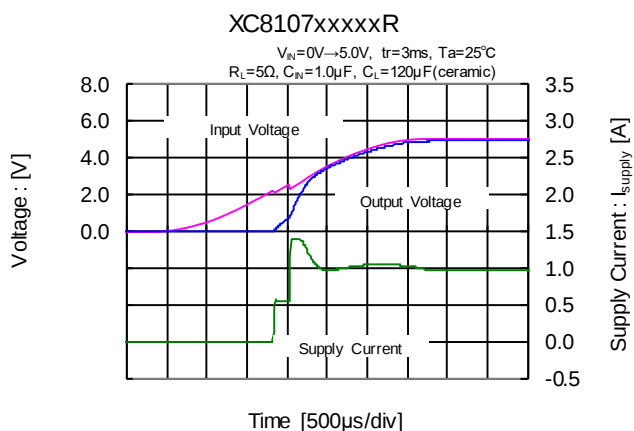
(38) UVLO Transient Response ( C_L=120\mu\text{F} )
