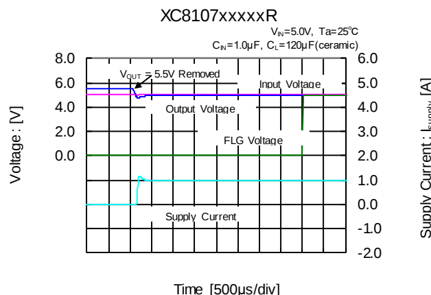
(42) Reverse Voltage Released Voltage ( C_L=120\mu\text{F} )
