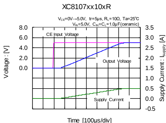
(24) turn-on Delay vs. Rise Time ( C_L=1.0\mu\text{F} )
