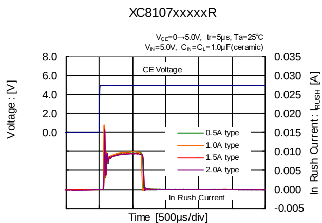
(43) CE Transient Response
