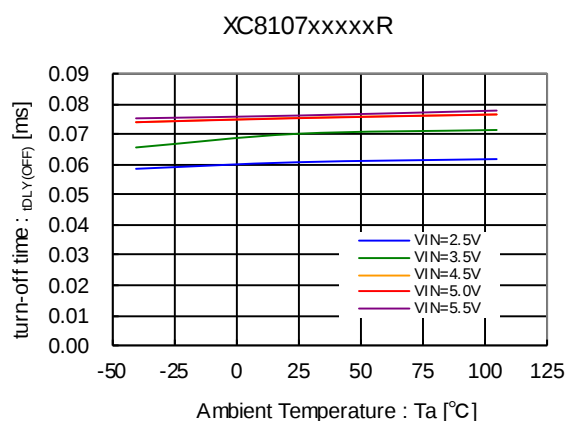
(20) turn-off time vs. Ambient Temperature
