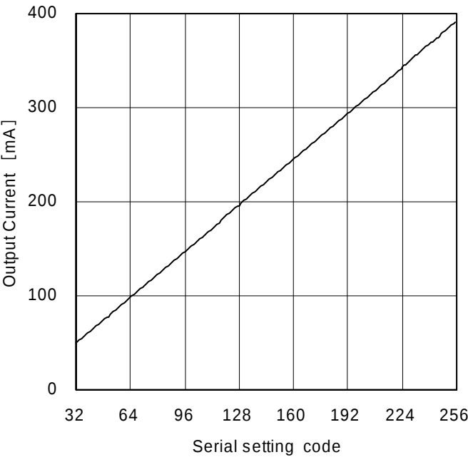
Figure 12. Output Current (Current driver block, RRNF = 1.0Ω , RL = 5.0Ω)
