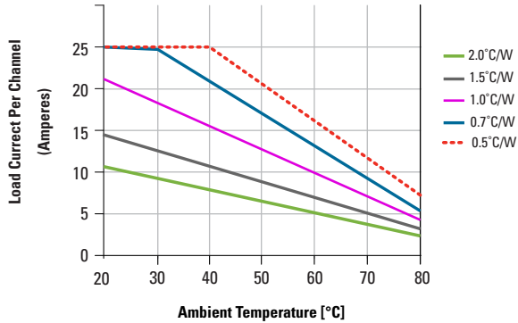
DERATE CURVES: 53TP IP20 25A
