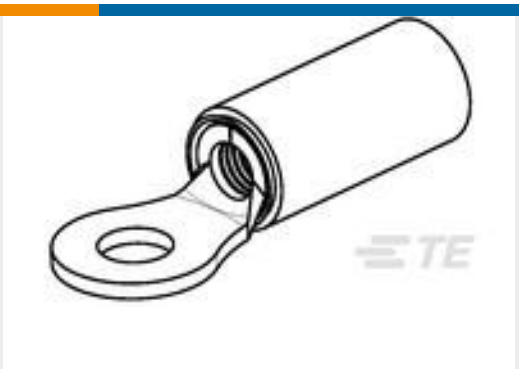
TE Part #1577646-1 TERMINAL RT PIDG PEEK STRATO 10 AWG
