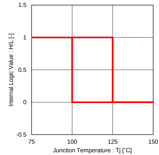
Figure 43 Thermal Shutdown
