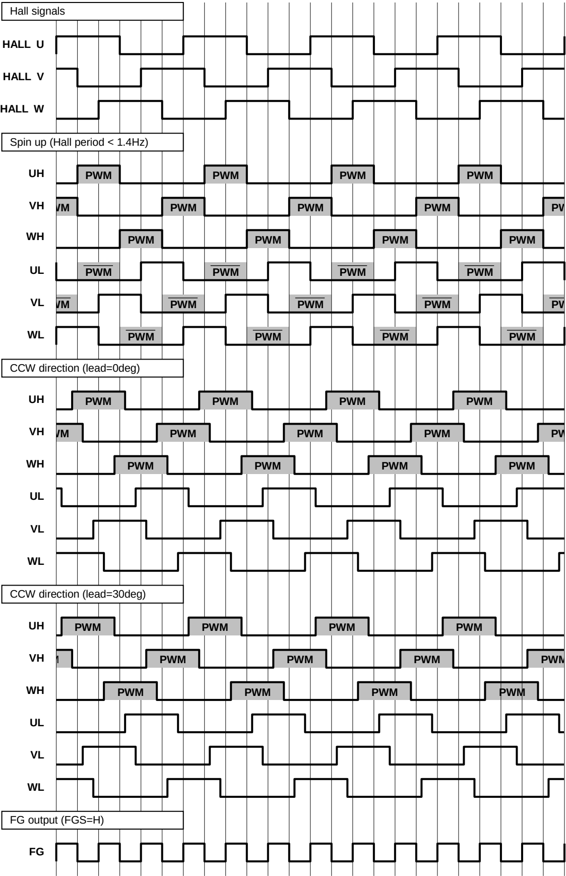
Timing Chart (CCW, SQB = H)
