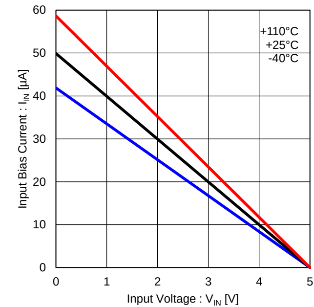
Figure 38. Input Bias Current (CCW, FGS, SQB)
