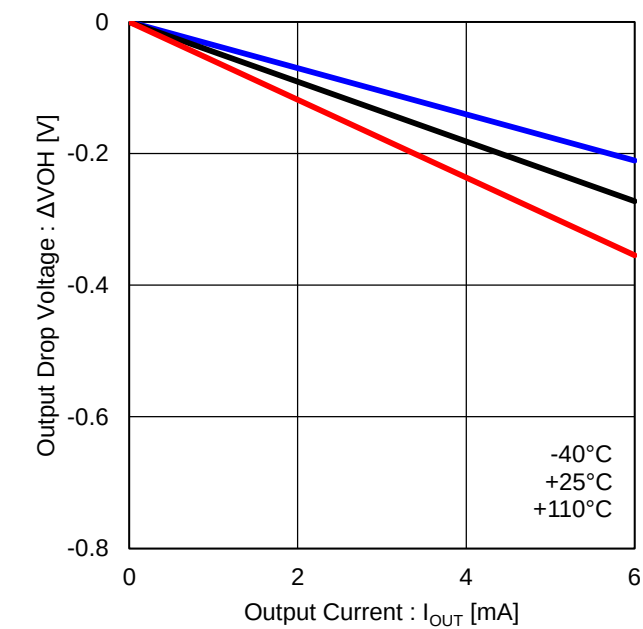
Figure 36. High Side Output Voltage (FG)
