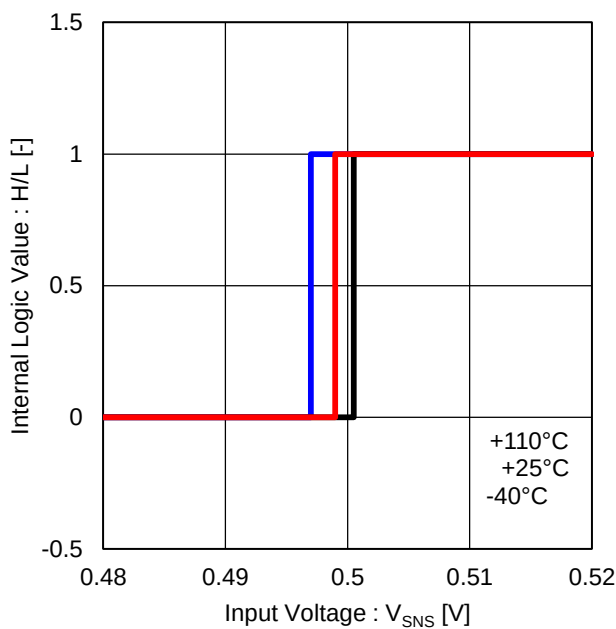
Figure 41. Current Limiter Input Threshold Voltage (SNS)
