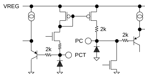
Figure 59. PC, PCT
