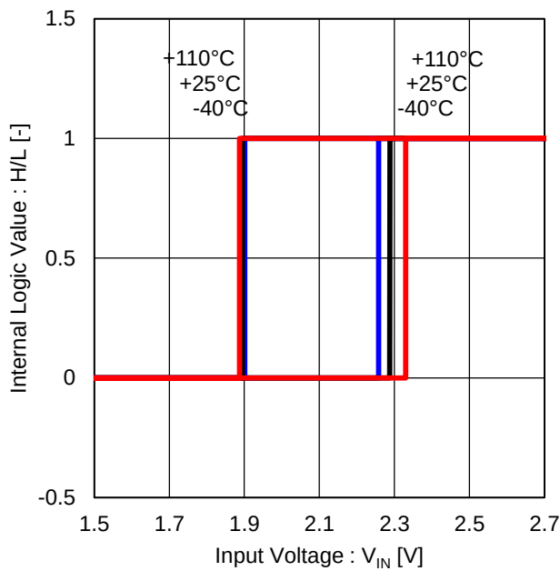
Figure 39. Input Threshold Voltage (CCW, FGS, SQB, FOB)
