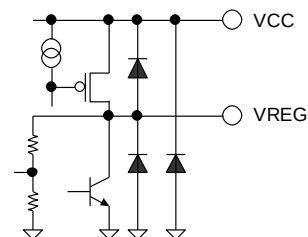
Figure 55. VREG, VCC
