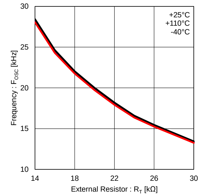
Figure 35. Carrier Frequency vs RT
