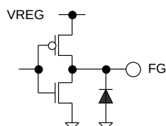
Figure 56. FG
