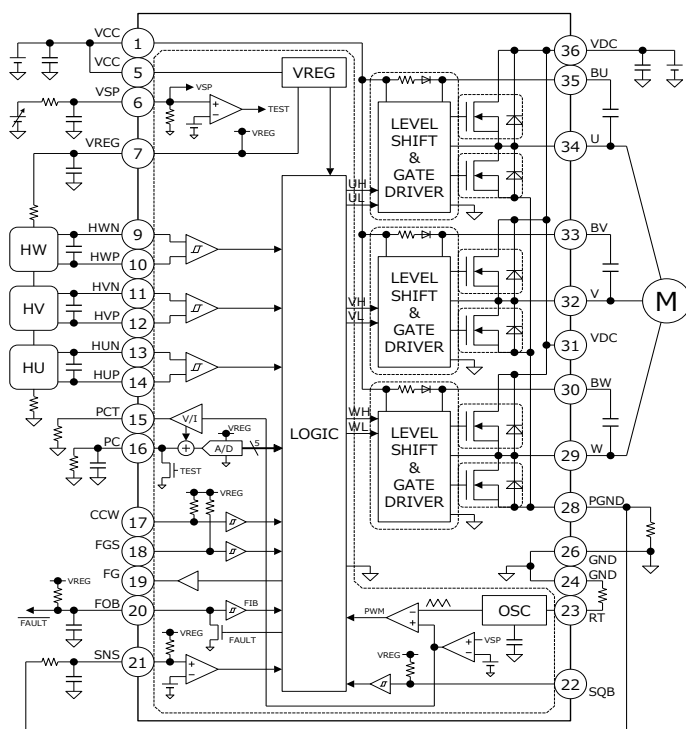
Figure 2. Block Diagram
