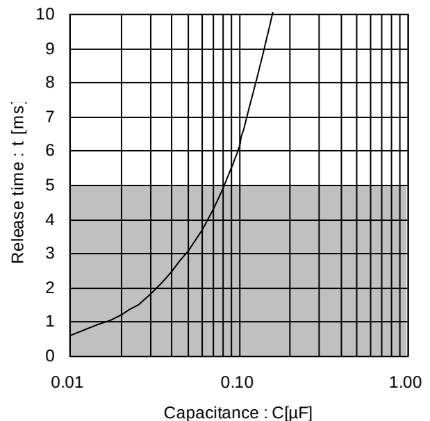
Figure 9. Release Time (Reference Data @R=100k \Omega )
