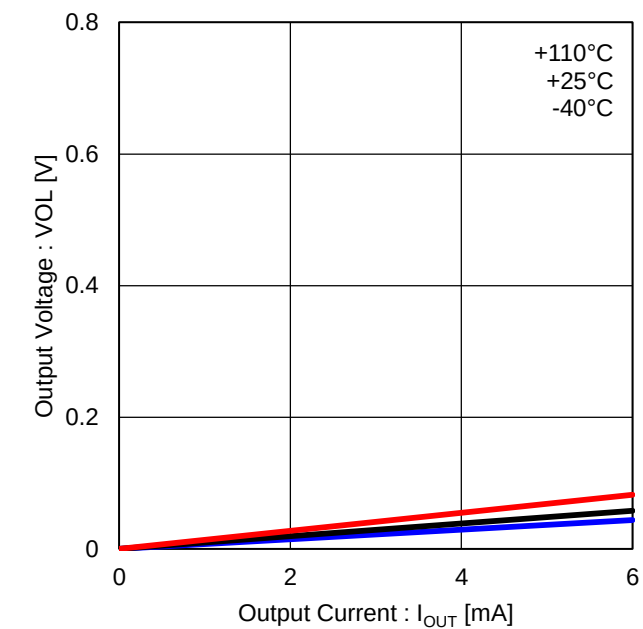
Figure 37. Low Side Output Voltage (FG)
