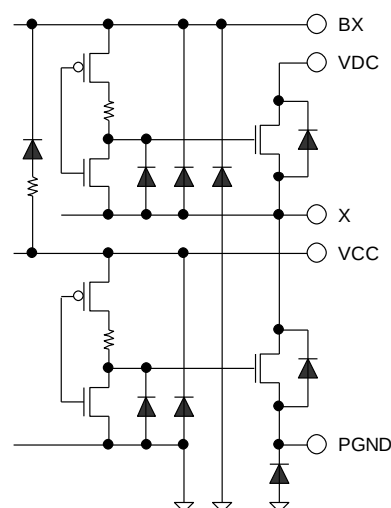
Figure 61. VCC, PGND, VDC, BX(BU/BV/BW), X(U/V/W)
