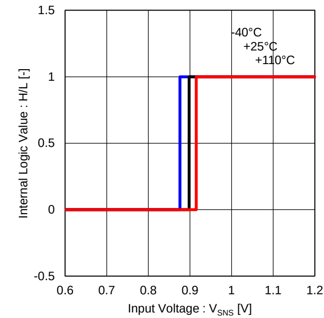
Figure 42. OCP Input Threshold Voltage (SNS)
