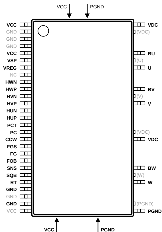
Figure 51. Dummy Pins
