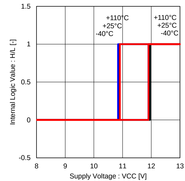
Figure 45. Under Voltage Lock Out (Low Side Drivers)
