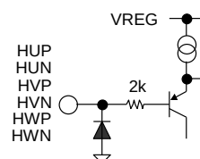
Figure 57. HXP, HXN
