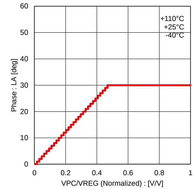
Figure 34. PC Voltage Normalized vs Lead Angle
