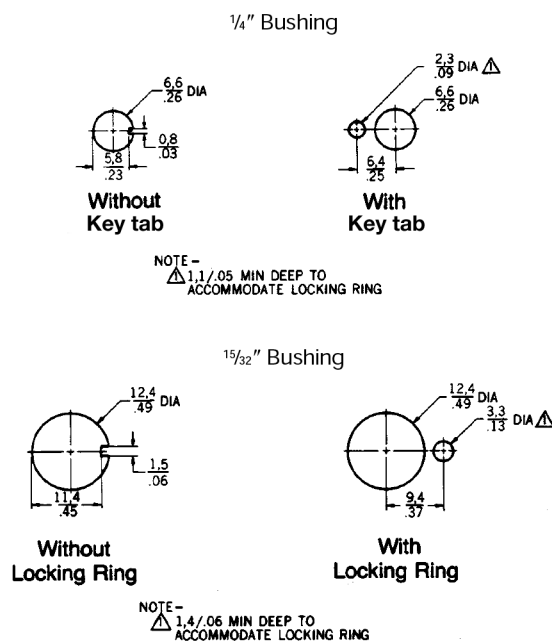
Figure 16. Panel Cutouts
