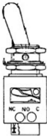
AT Series Toggle Sw itch, 2 pole, 2 position, Solder T2 type terminal, Locking Lever
