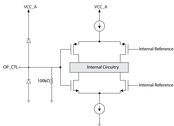
Figure 3-6: OP_CTL
