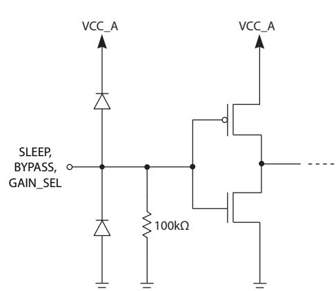
Figure 3-4: SLEEP, BYPASS, and GAIN_SEL Circuits
