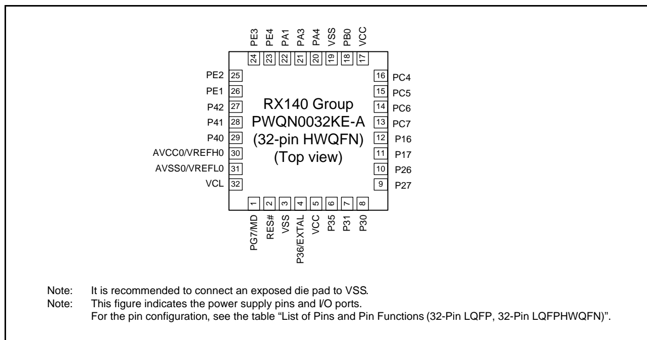
Figure 1.8 Pin Assignments of the 32-Pin HWQFN
