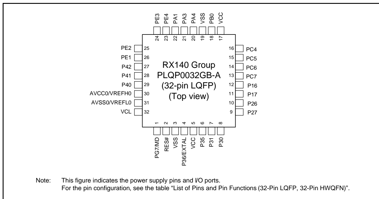
Figure 1.7 Pin Assignments of the 32-Pin LQFP
