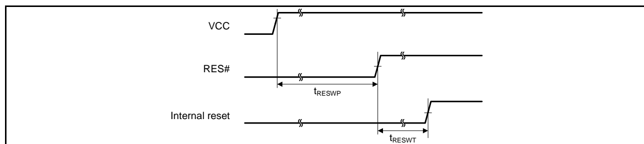
Figure 2.22 Reset Input Timing at Power-On
