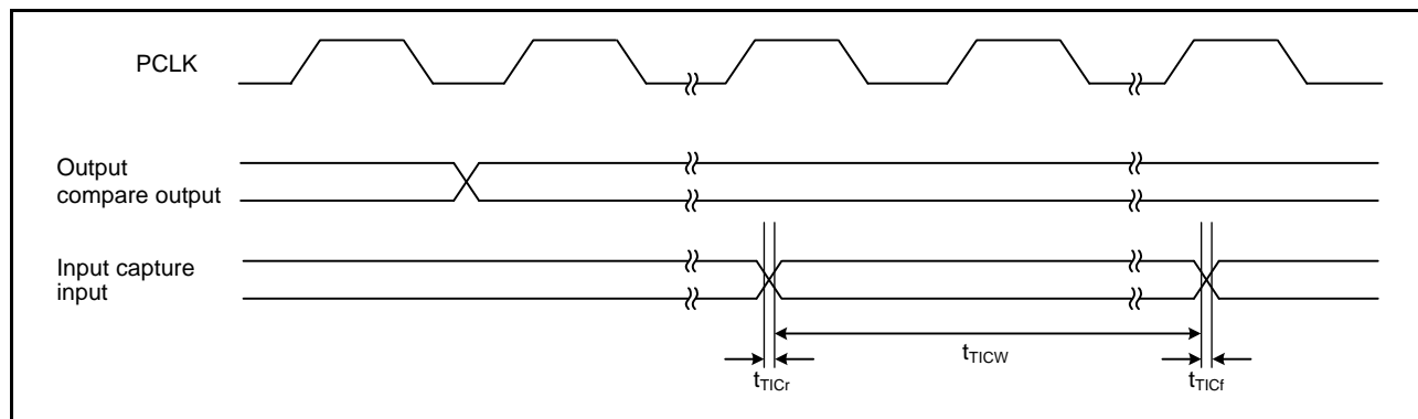
Figure 2.30 MTU2 Input/Output Timing
