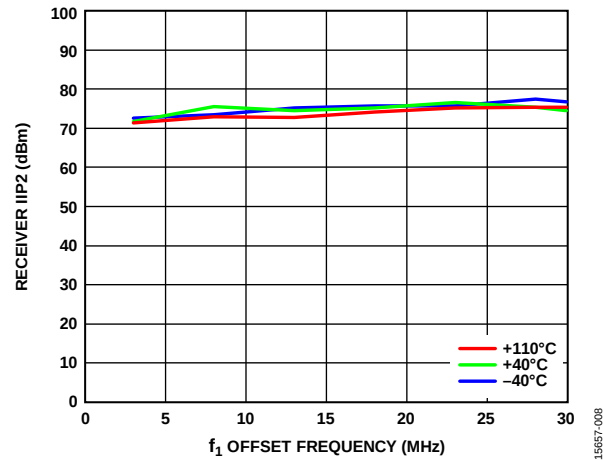
Figure 67. Receiver IIP2 vs. f_1 Offset Frequency, 2600 MHz LO, 0 dB Attenuation, 40 MHz RF Bandwidth, f_2 = f_1 + 1 MHz, 122.88 MSPS Sample Rate
