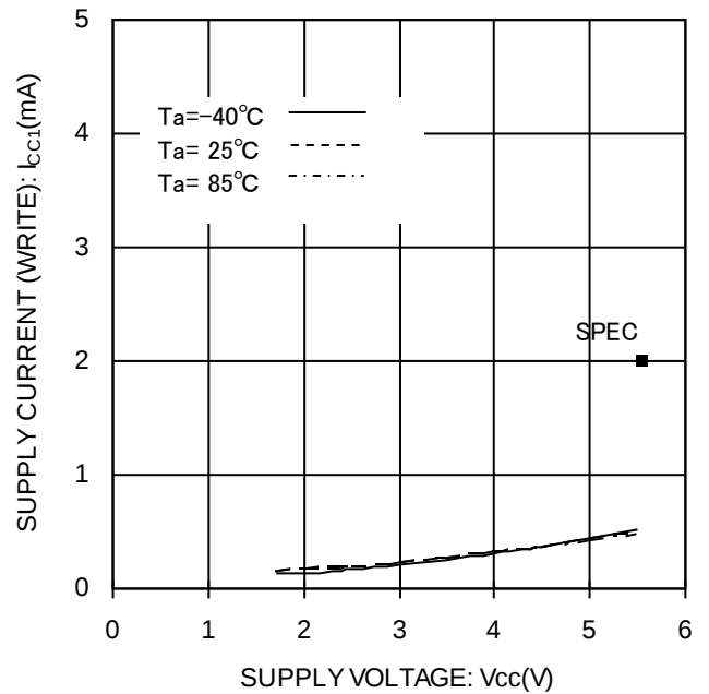
Figure 15. Supply Current (WRITE) vs Supply Voltage ( f_{SK} = 3 MHz )
