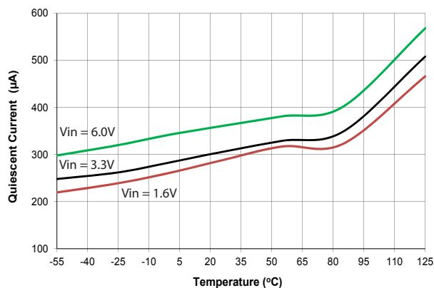
Quiescent Current
