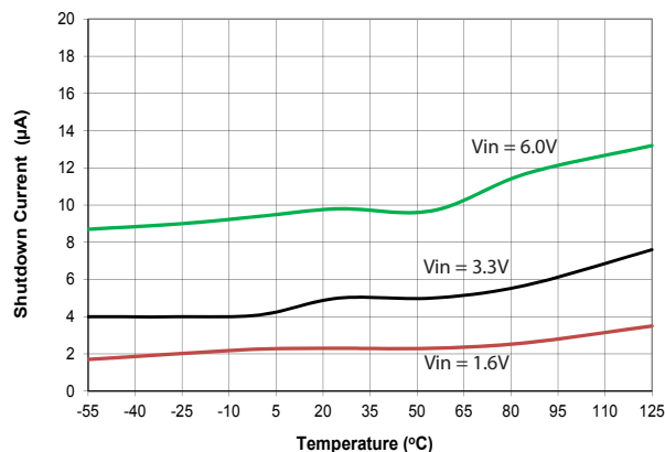
Shutdown Current
