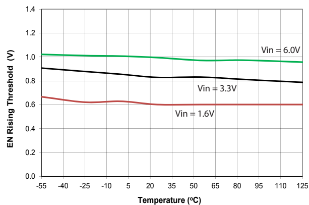
ENABLE Rising Threshold
