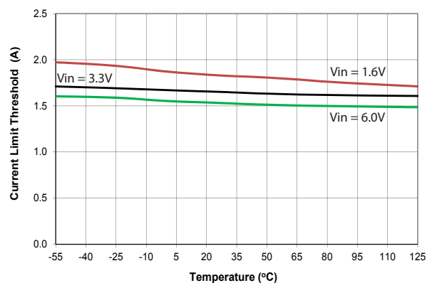
Current Limit Threshold
