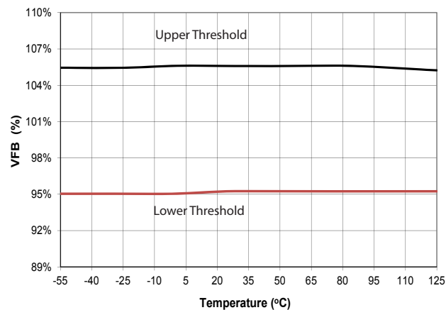
PG Threshold
